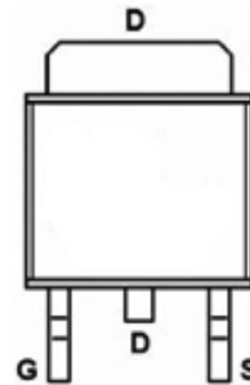
pin assignment
