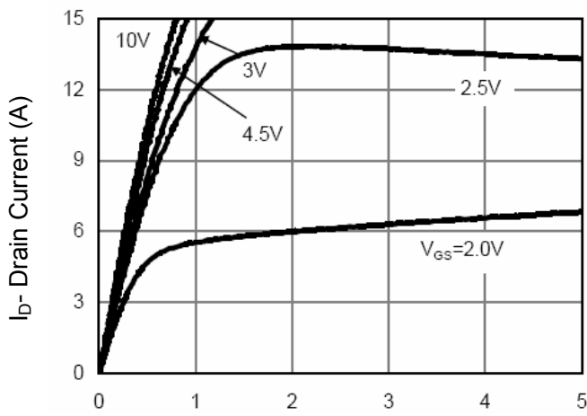
Figure 5 Output Characteristics
