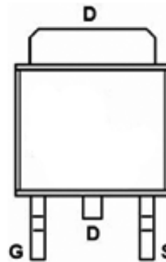
pin assignment
